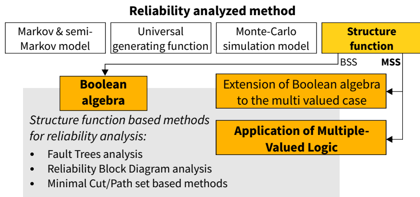
Figure 1: Classification of methods for MSS reliability analysis
