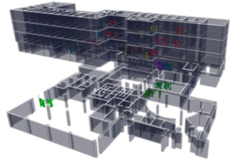
Figure 3: PedSim simulation tool: Simulation of pedestrian movement
